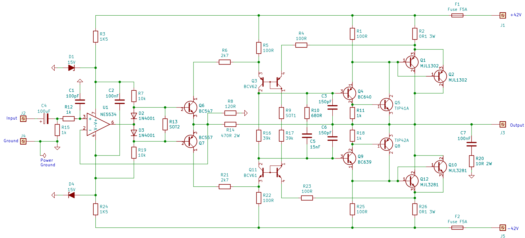
Figure 5 from 'Audio Amplifier with Defined Output Impedance' by John Howard, available at robinet.co.uk Licensed under a Creative Commons Attribution-NonCommercial-ShareAlike 4.0 International License
